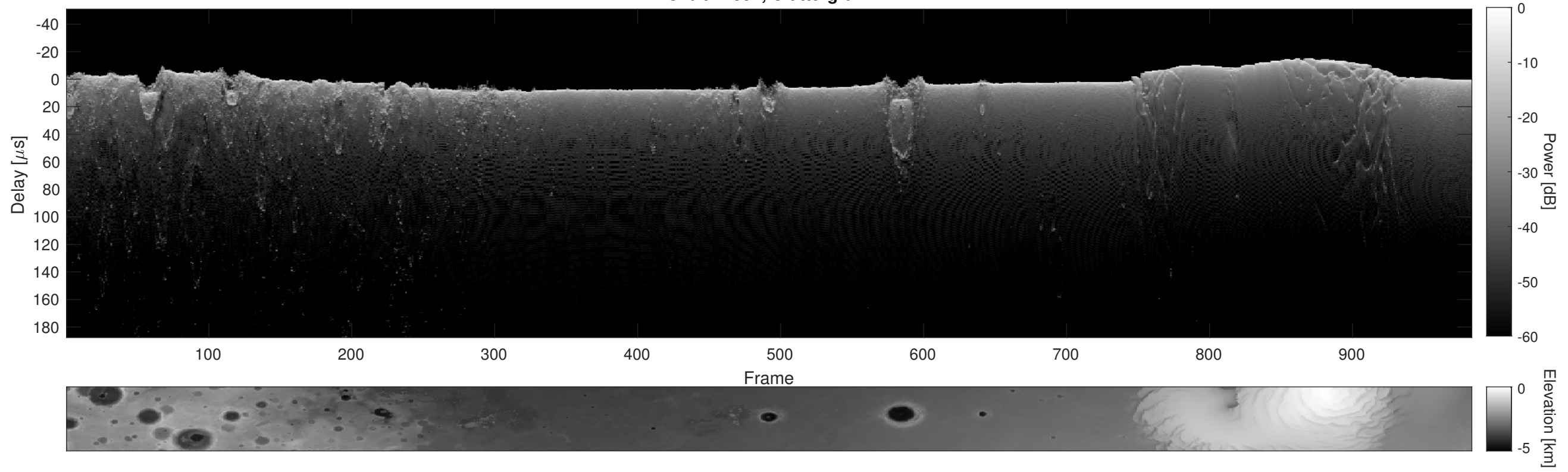
Orbit 22597, Cluttergram
