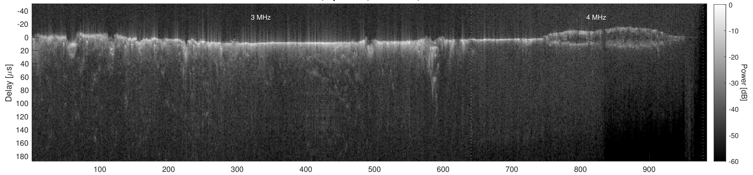
Orbit 22597, Cluttergram
