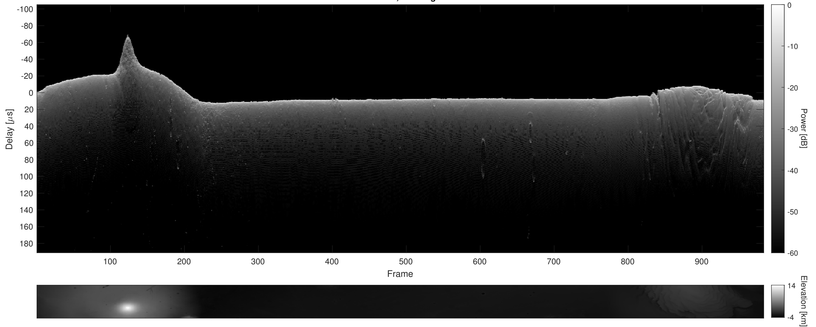
Orbit 22599, Cluttergram
