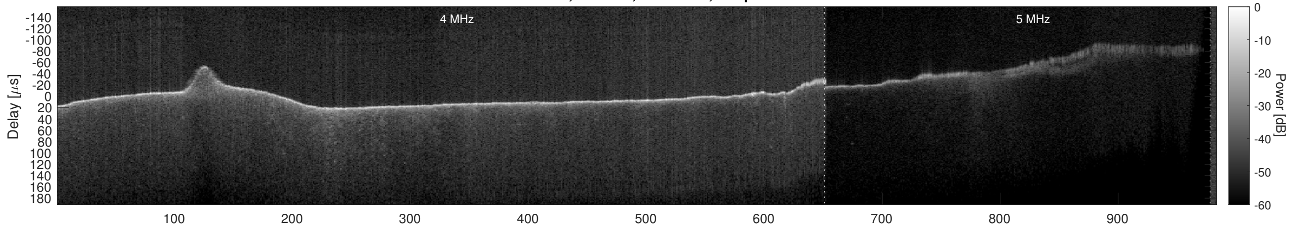
Orbit 22599, Window, Channel 1, Optimized
