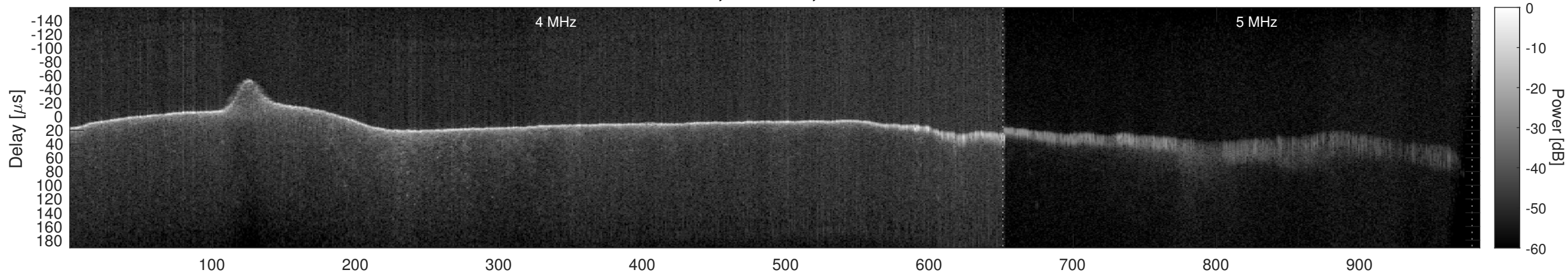
Orbit 22599, Window, Channel 1, Chapman
