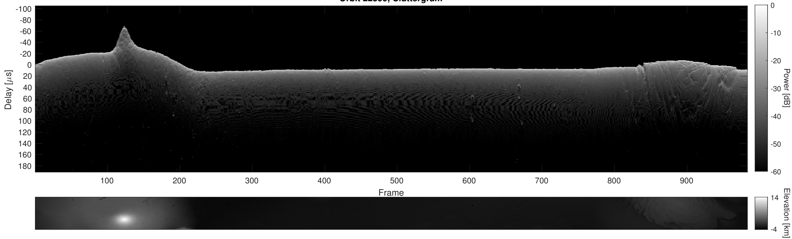
Orbit 22599, Cluttergram
