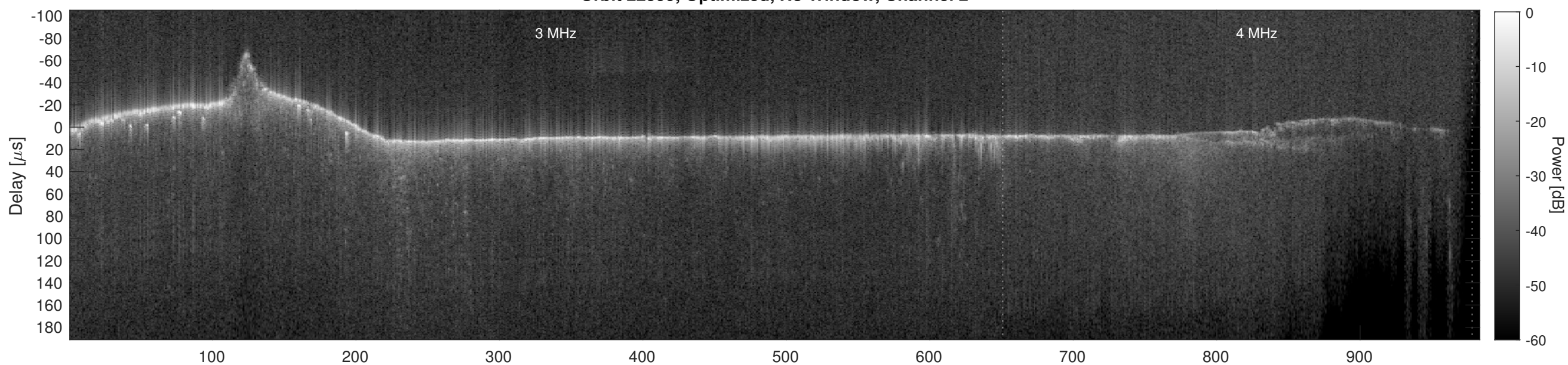
Orbit 22599, Cluttergram
