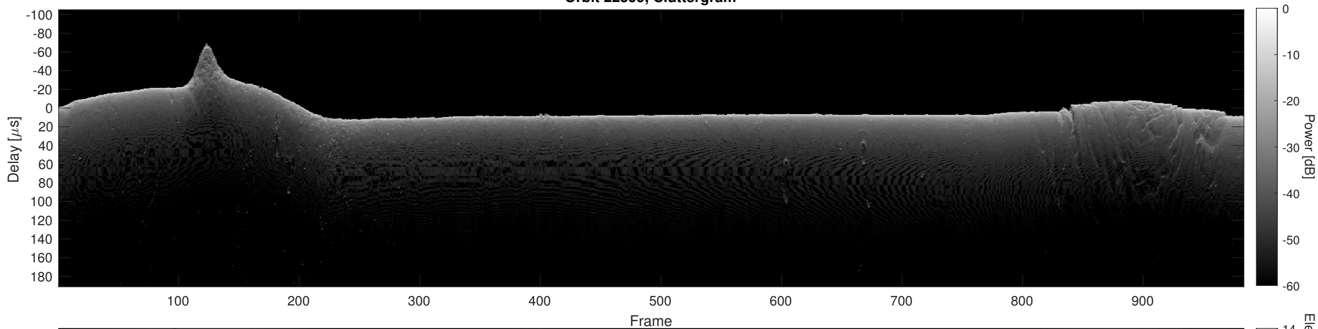
Orbit 22599, Cluttergram
