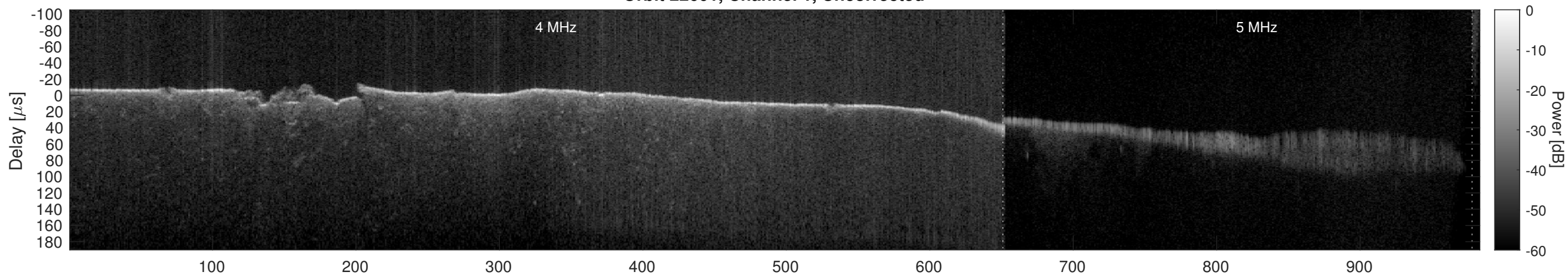
Orbit 22601, Window, Channel 1, Chapman
