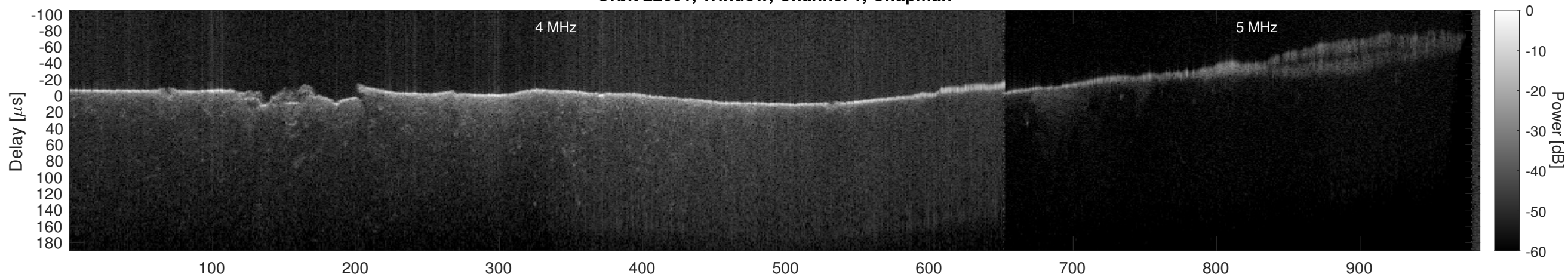
Orbit 22601, Window, Channel 1, Optimized
