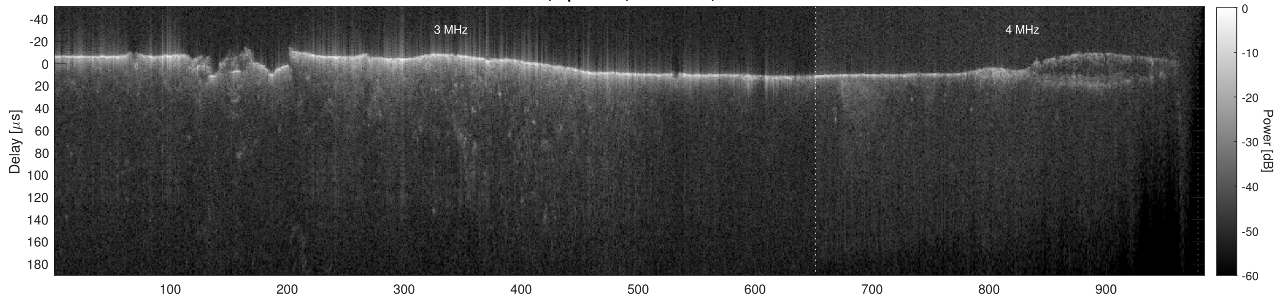
Orbit 22601, Cluttergram
