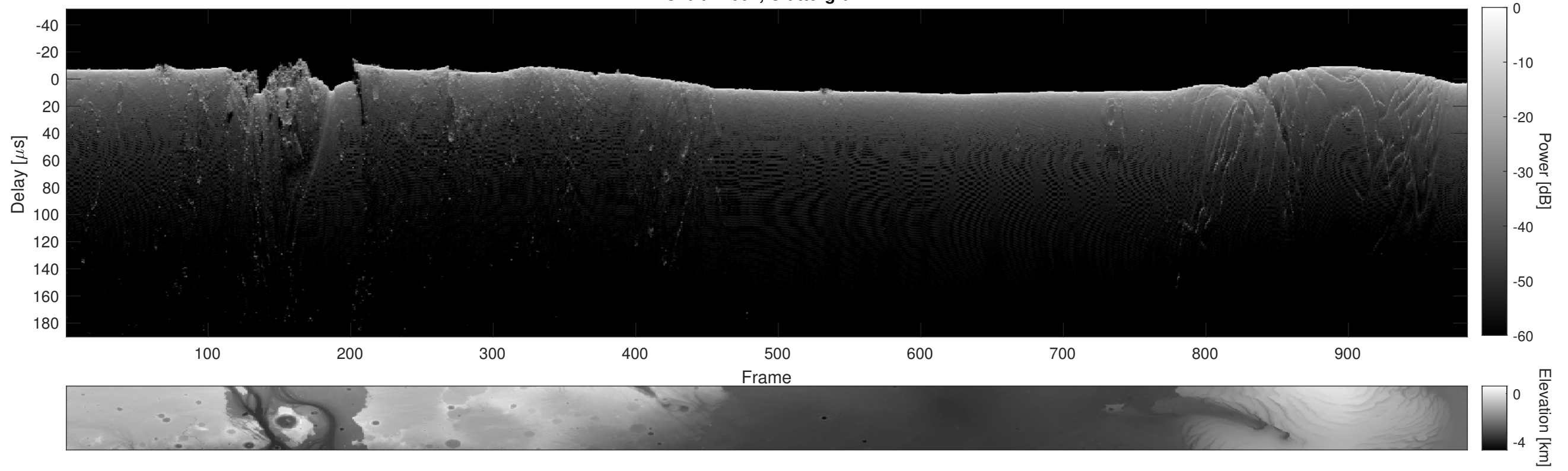
Orbit 22601, Cluttergram
