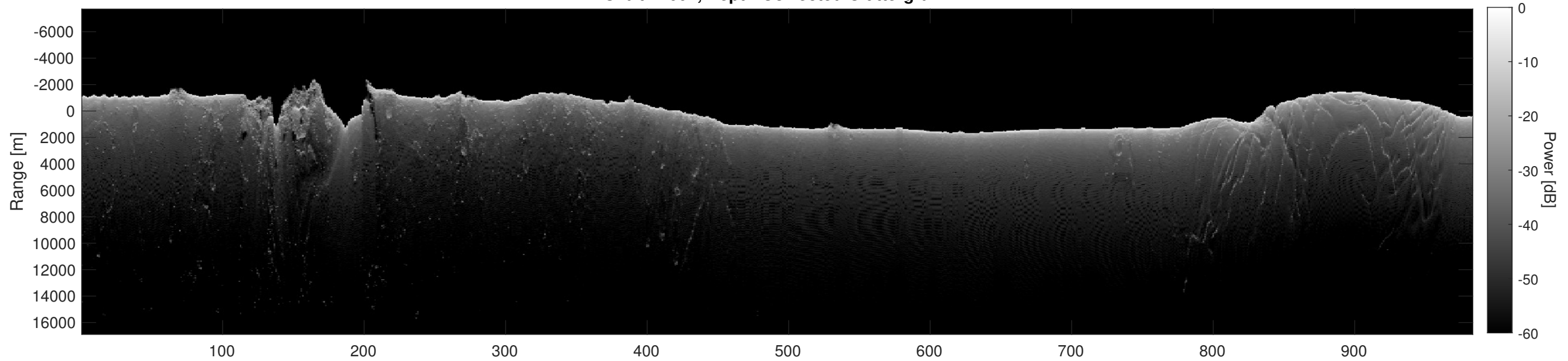
Orbit 22601, Depth-Corrected Cluttergram
