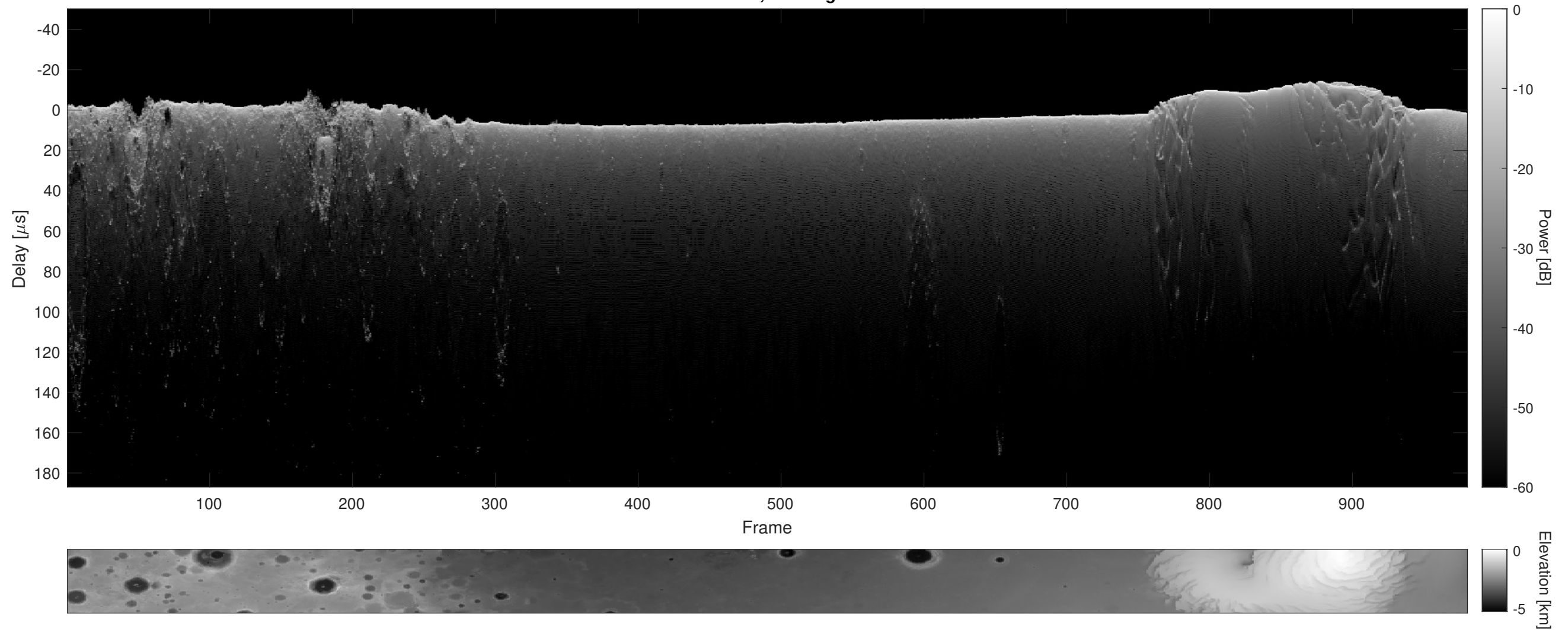
Orbit 22604, Cluttergram
