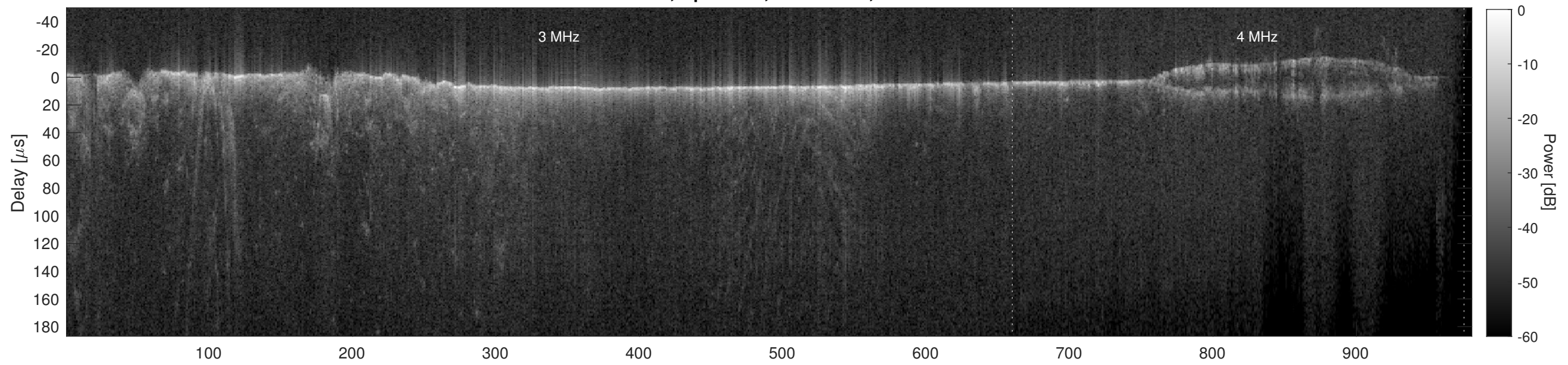
Orbit 22604, Cluttergram
