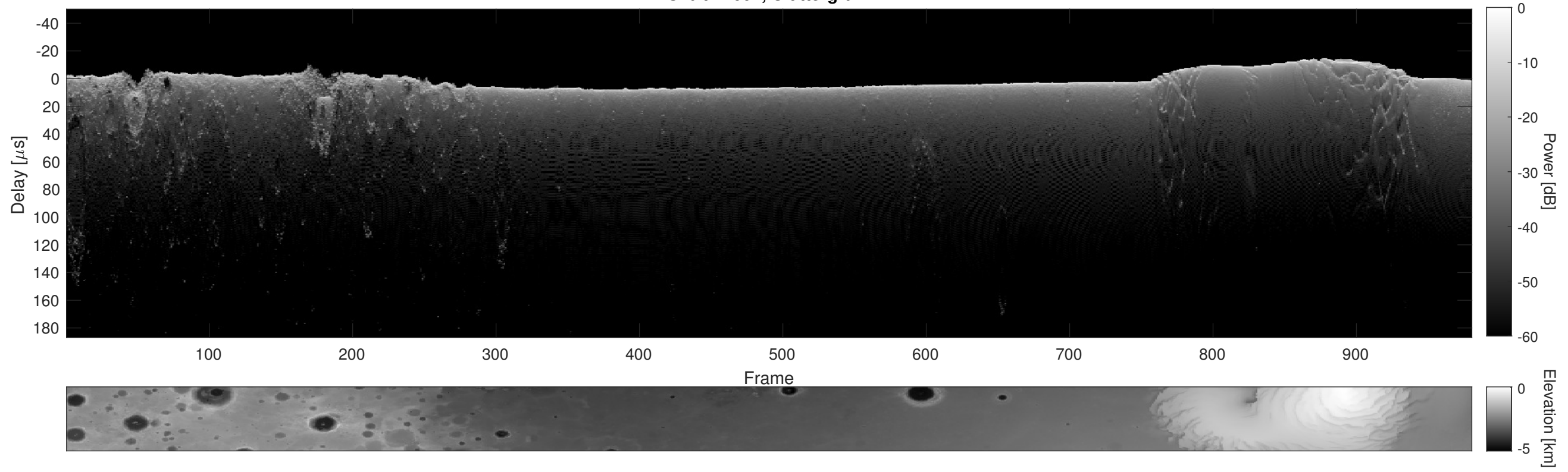
Orbit 22604, Cluttergram
