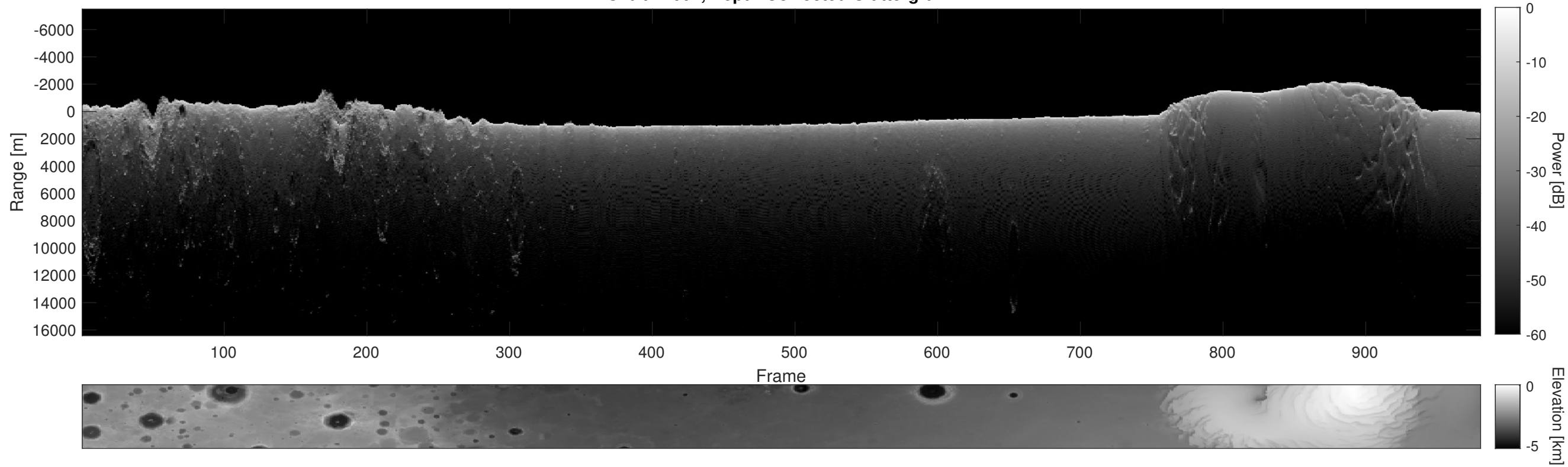
Orbit 22604, Depth-Corrected Cluttergram
