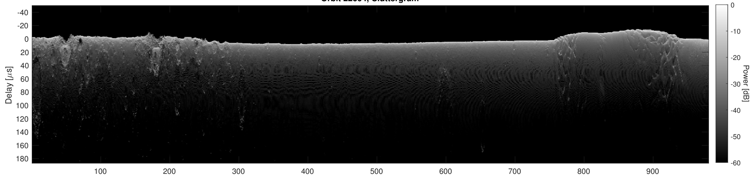
Orbit 22604, Cluttergram
