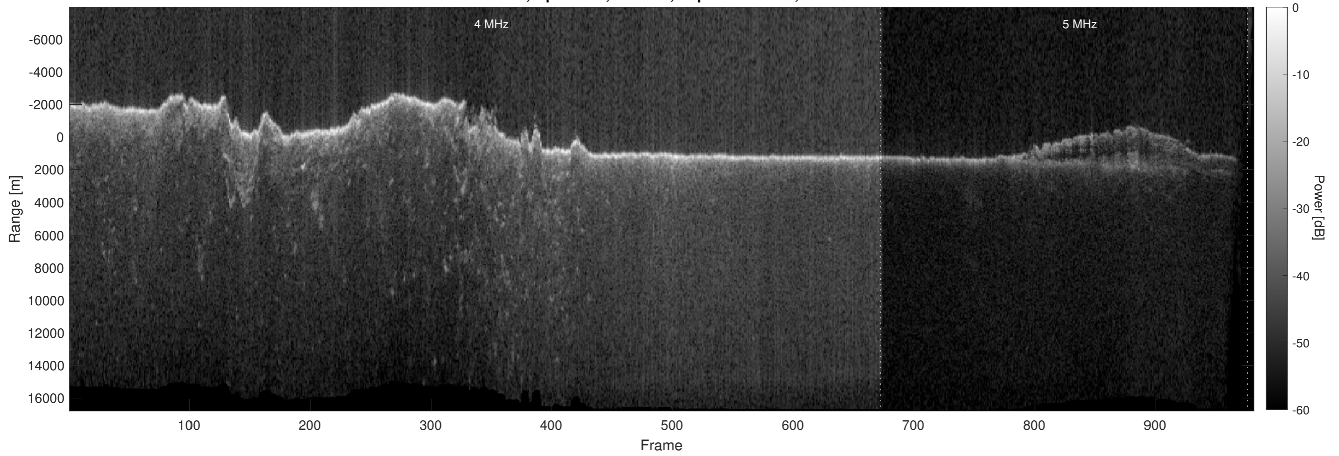
Orbit 22607, Optimized, Window, Depth-Corrected, Channel 2
