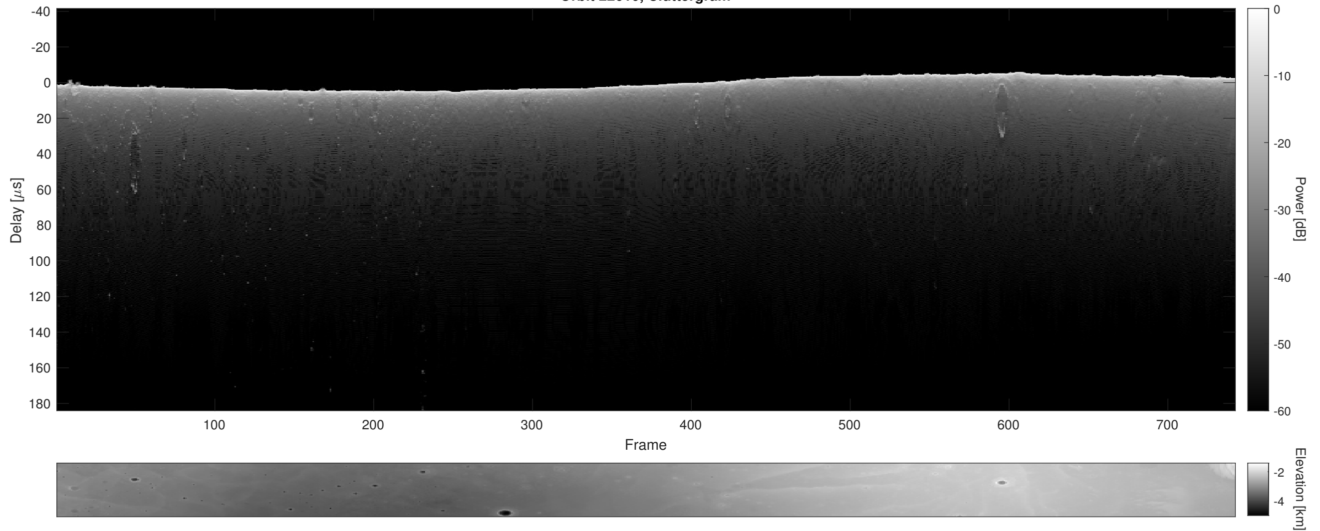
Orbit 22610, Cluttergram
