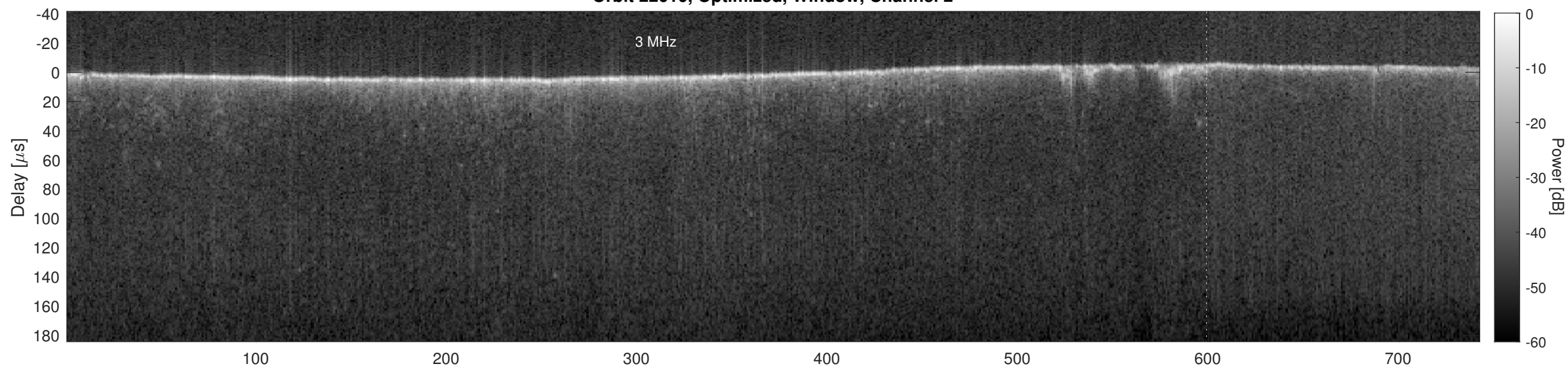
Orbit 22610, Cluttergram
