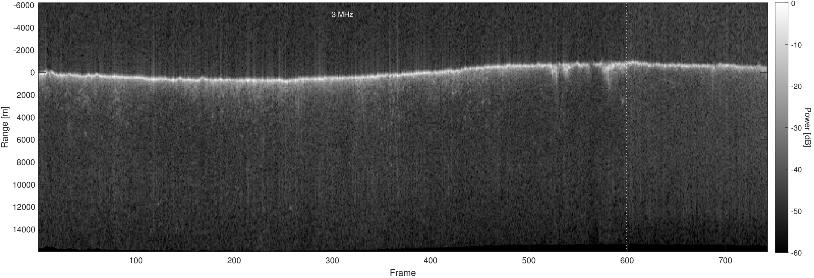
Orbit 22610, Optimized, Window, Depth-Corrected, Channel 2
