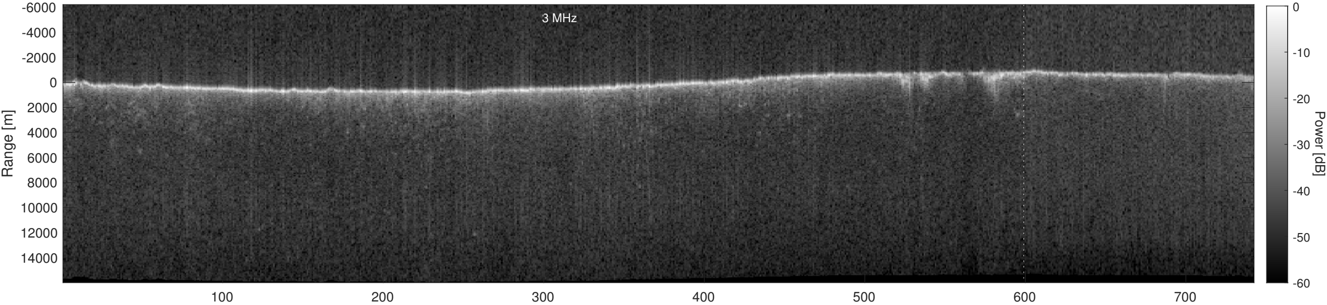
Orbit 22610, Depth-Corrected Cluttergram
