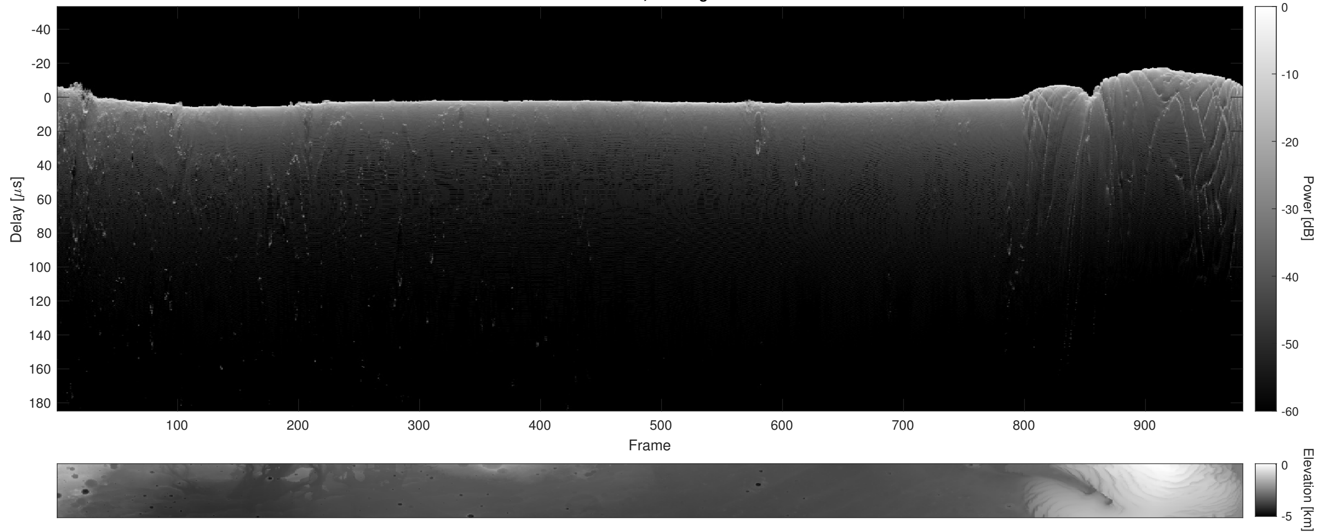
Orbit 22615, Cluttergram
