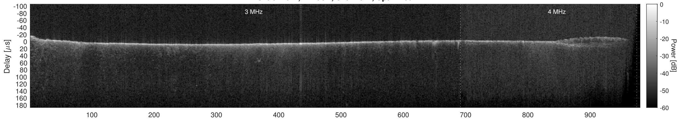
Orbit 22617, Cluttergram
