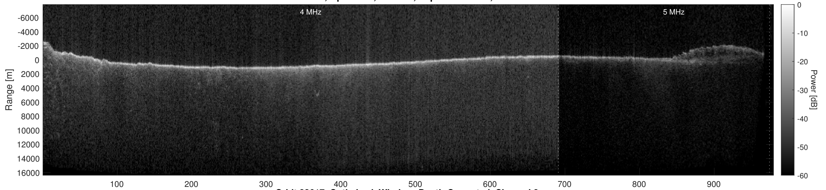
Orbit 22617, Optimized, Window, Depth-Corrected, Channel 2
