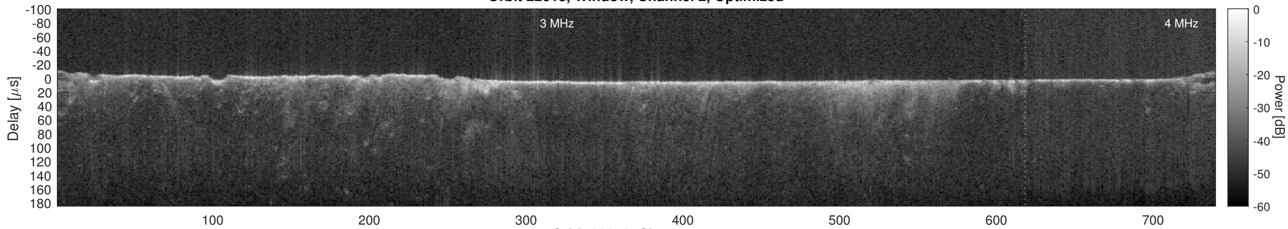
Orbit 22618, Cluttergram
