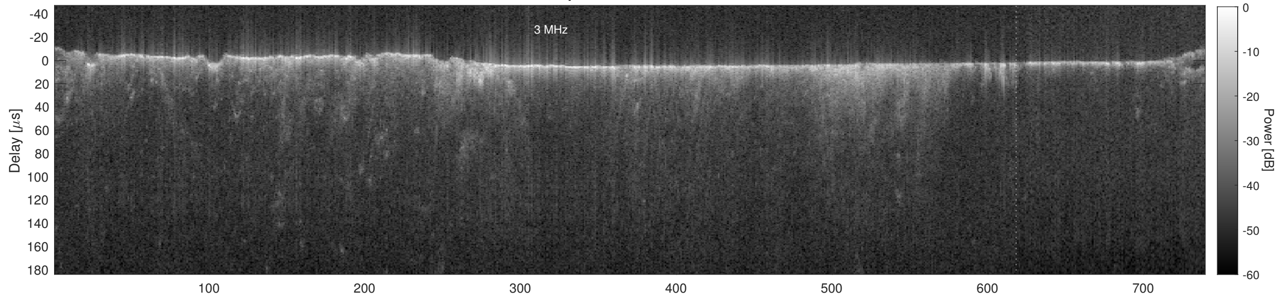
Orbit 22618, Cluttergram
