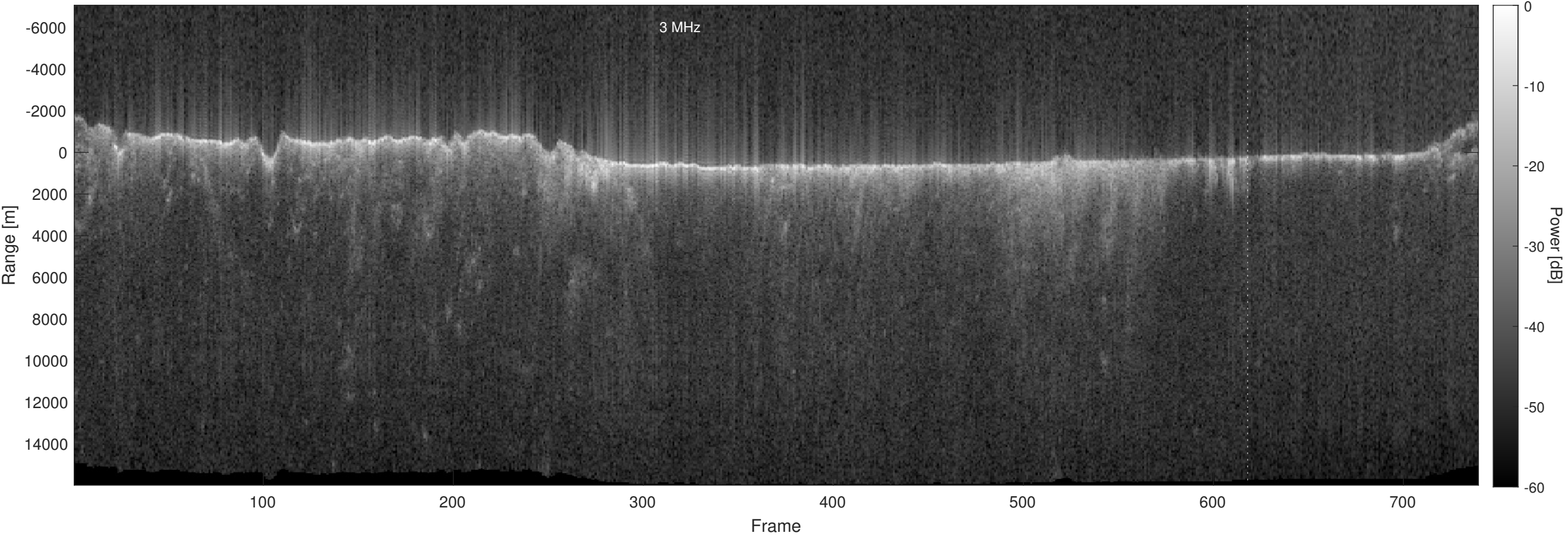
Orbit 22618, Optimized, No Window, Depth-Corrected, Channel 2
