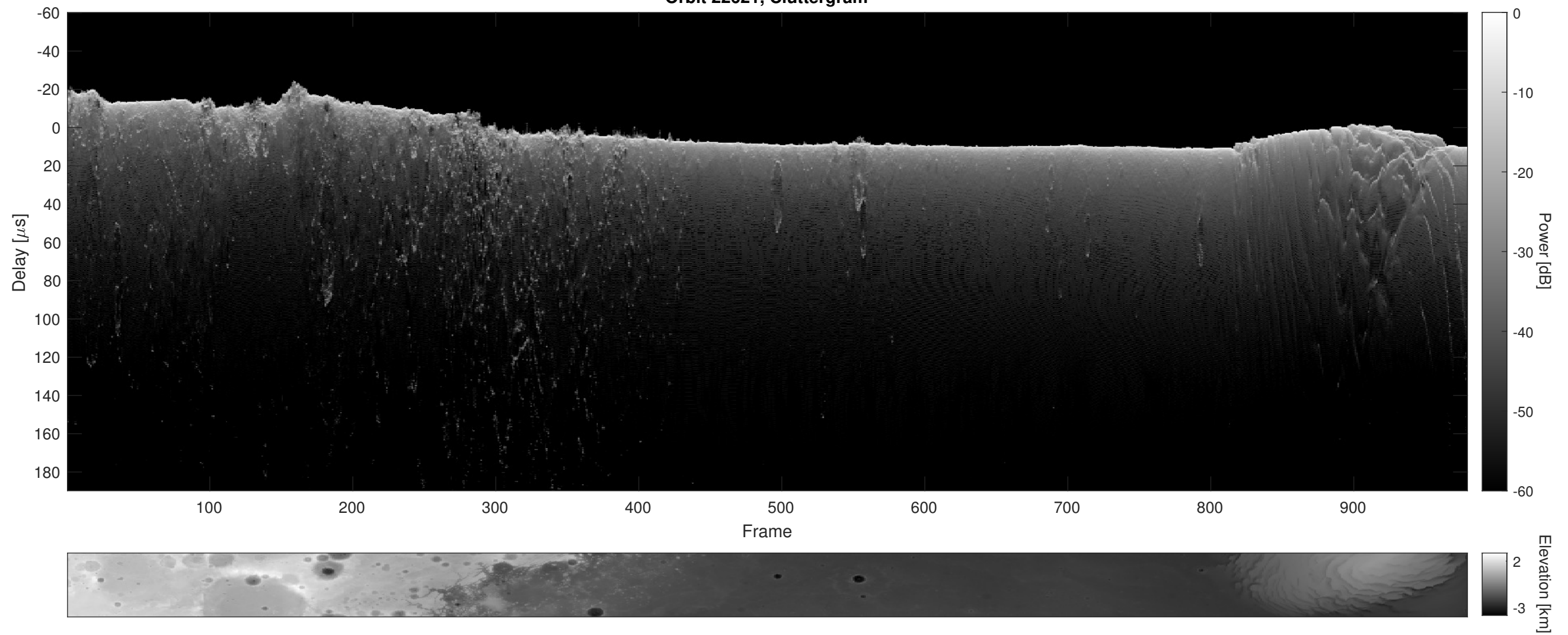
Orbit 22621, Cluttergram
