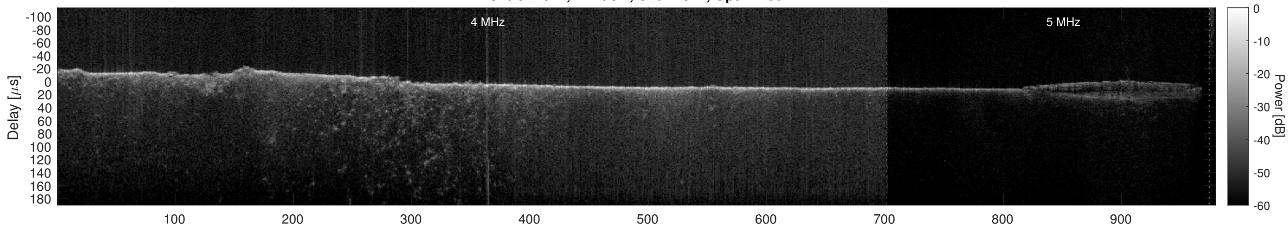
Orbit 22621, Cluttergram
