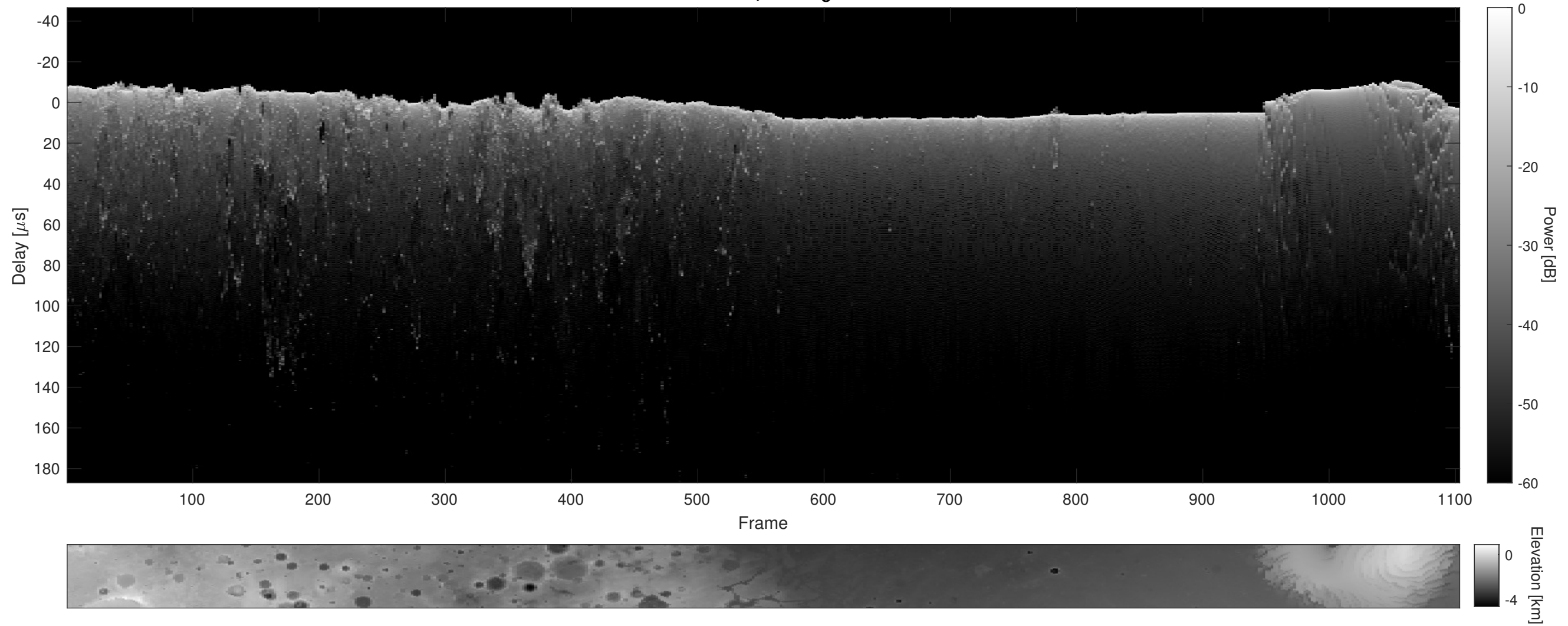
Orbit 22625, Cluttergram
