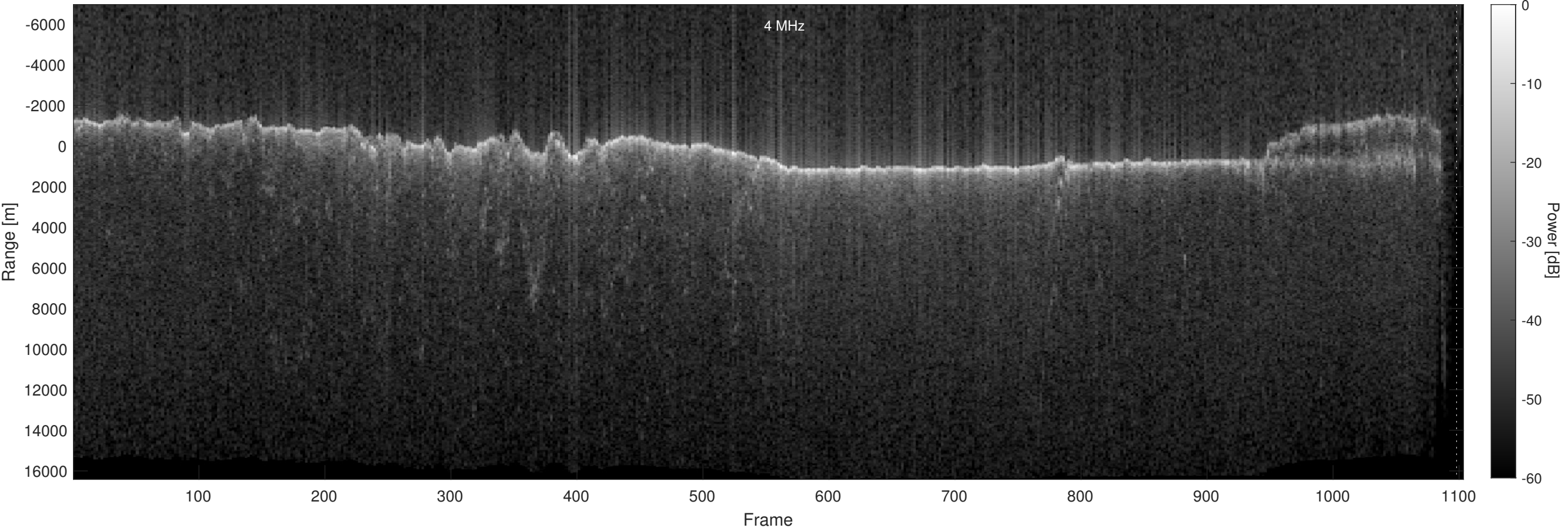
Orbit 22625, Optimized, No Window, Depth-Corrected, Channel 2
