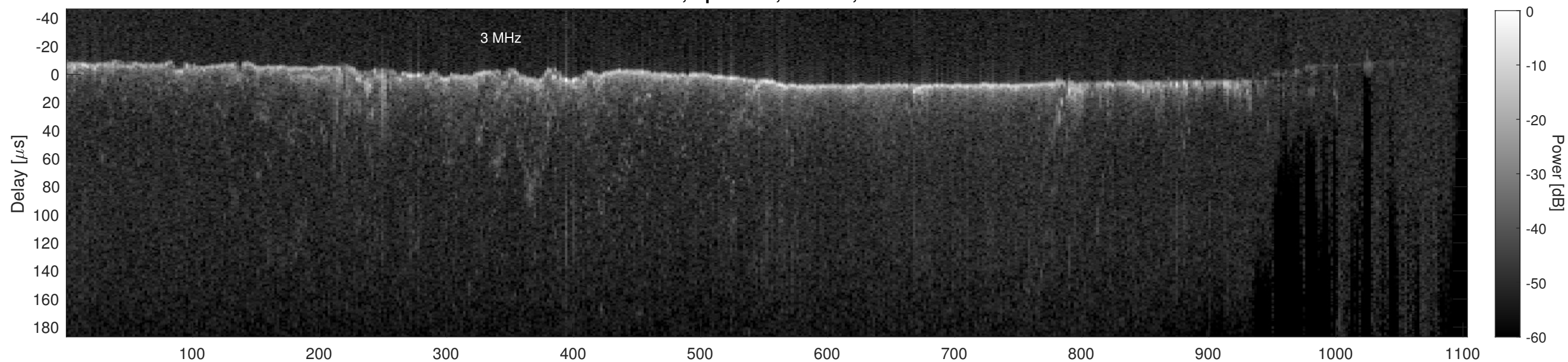
Orbit 22625, Cluttergram
