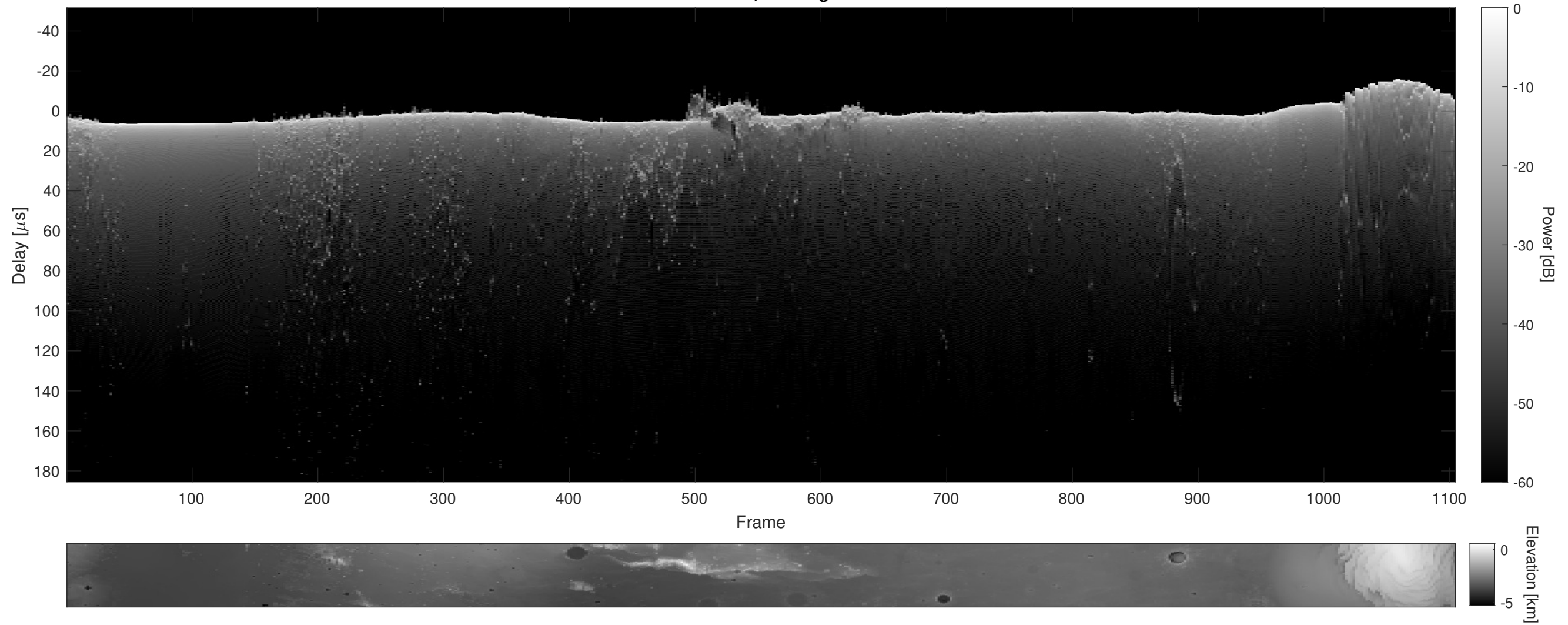
Orbit 22627, Cluttergram
