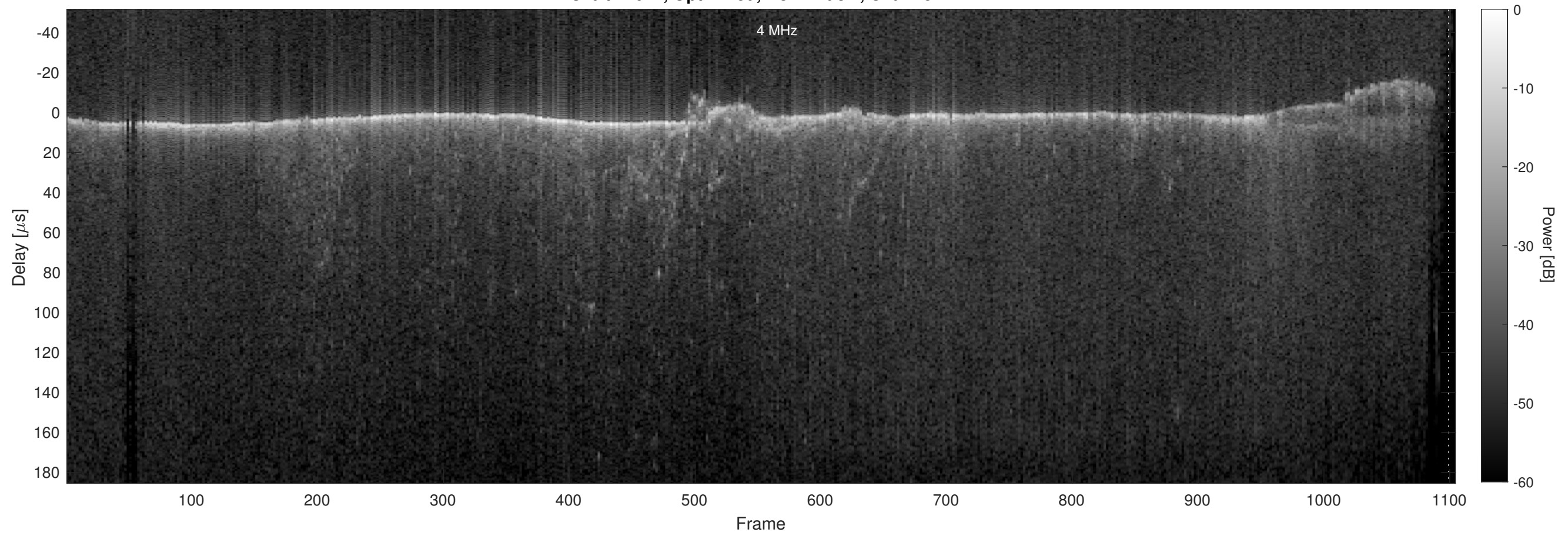
Orbit 22627, Optimized, No Window, Channel 2
