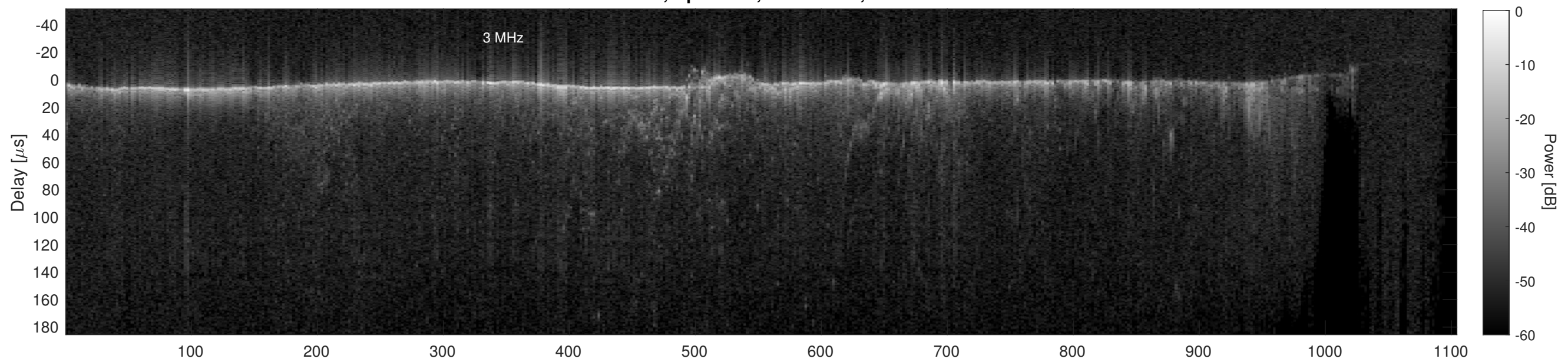
Orbit 22627, Cluttergram
