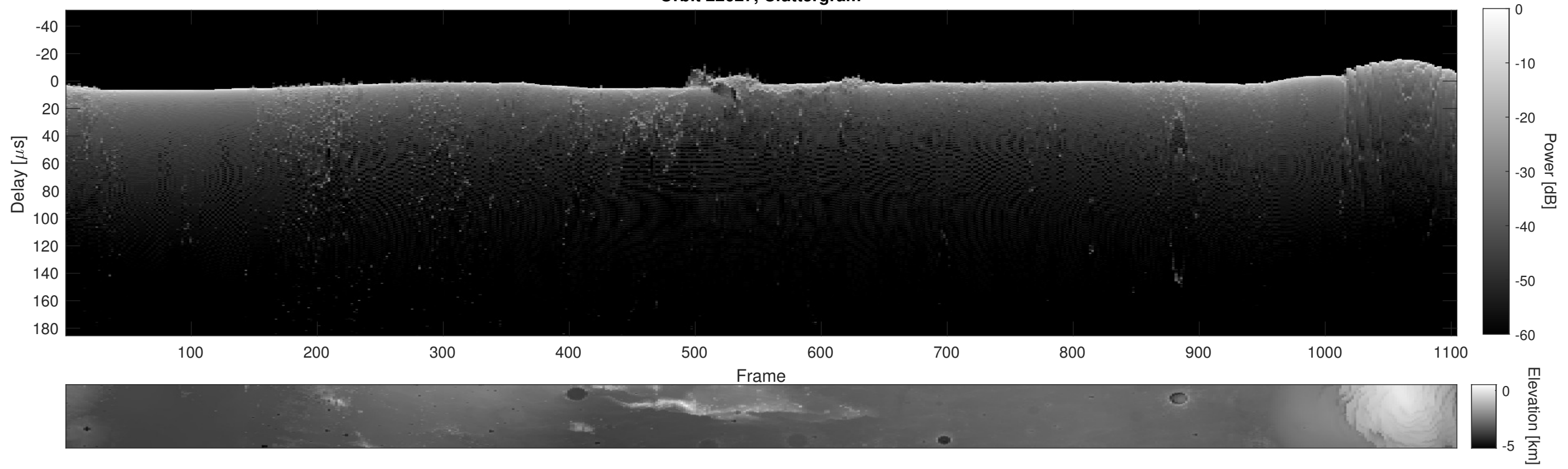
Orbit 22627, Cluttergram
