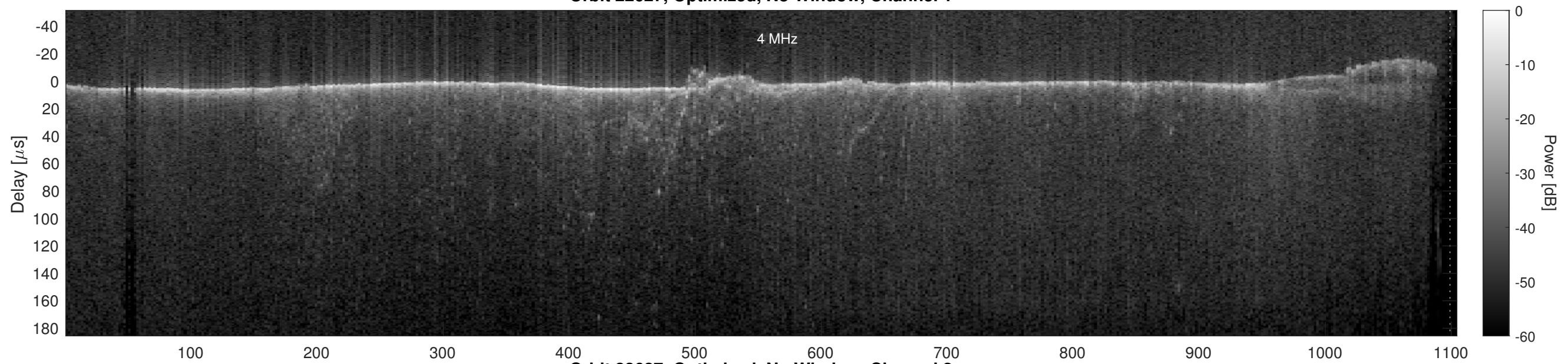
Orbit 22627, Optimized, No Window, Channel 2
