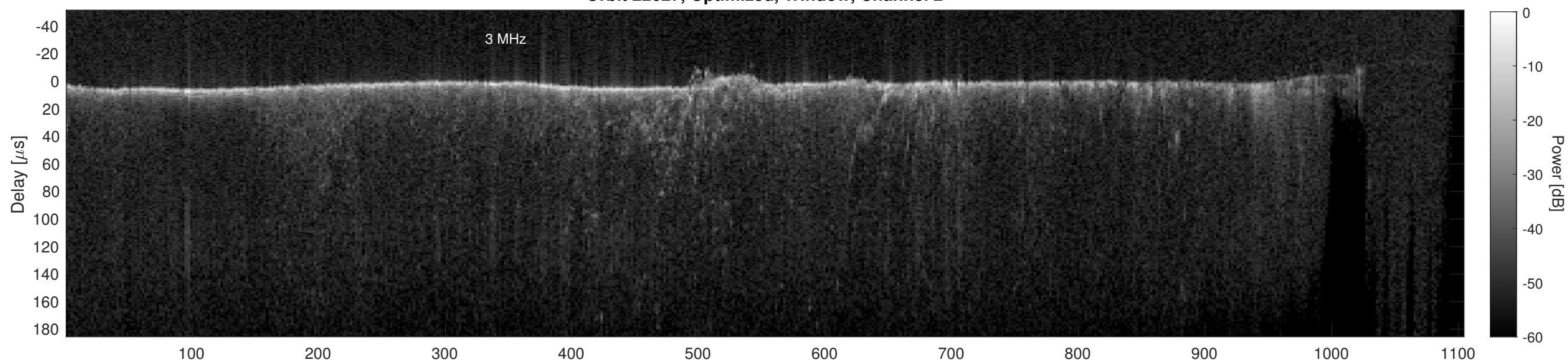
Orbit 22627, Cluttergram
