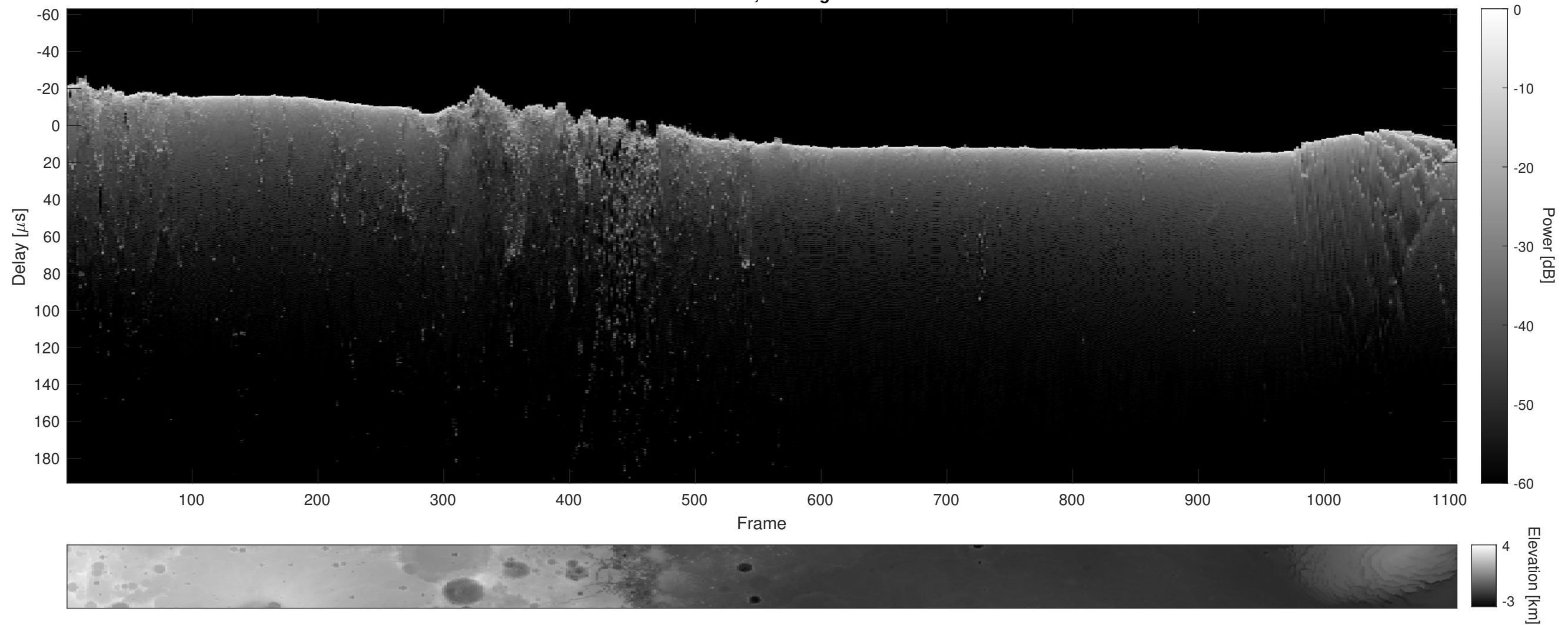
Orbit 22628, Cluttergram
