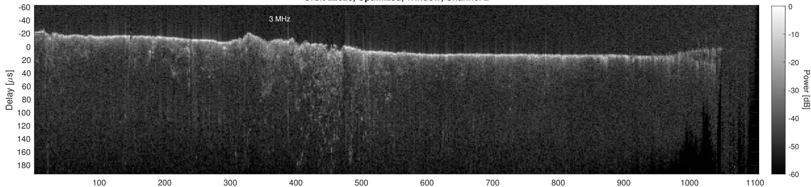
Orbit 22628, Cluttergram
