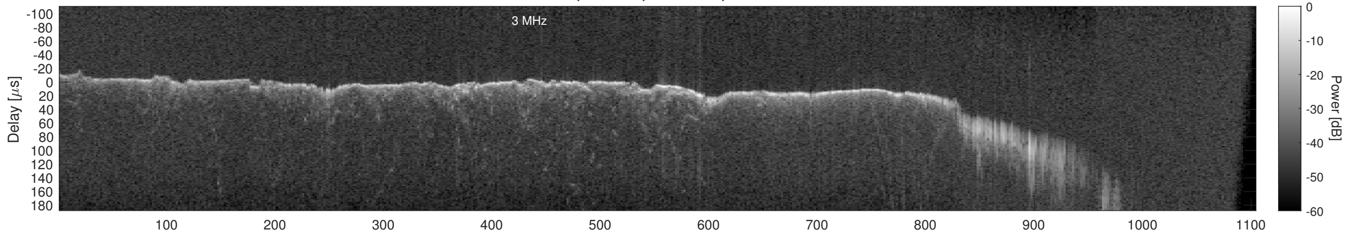
Orbit 22632, Window, Channel 2, Chapman
