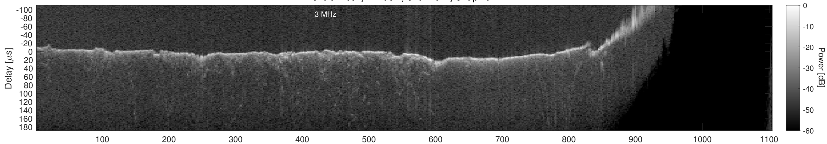
Orbit 22632, Window, Channel 2, Optimized
