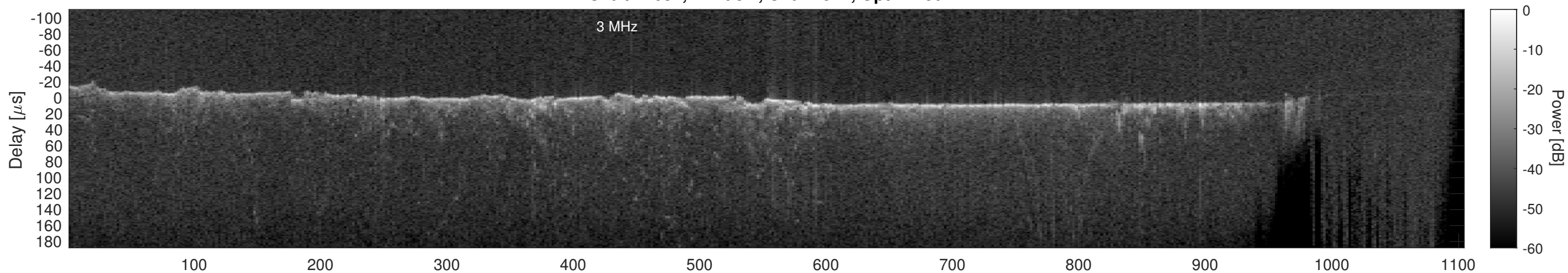
Orbit 22632, Cluttergram
