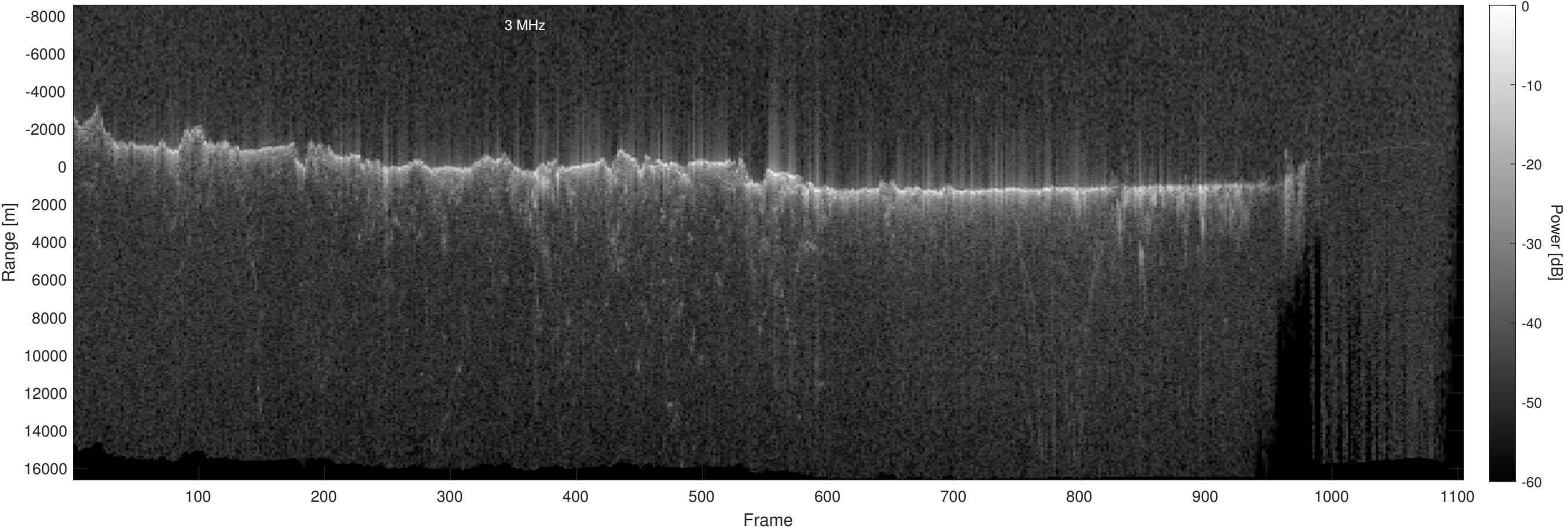
Orbit 22632, Optimized, No Window, Depth-Corrected, Channel 2
