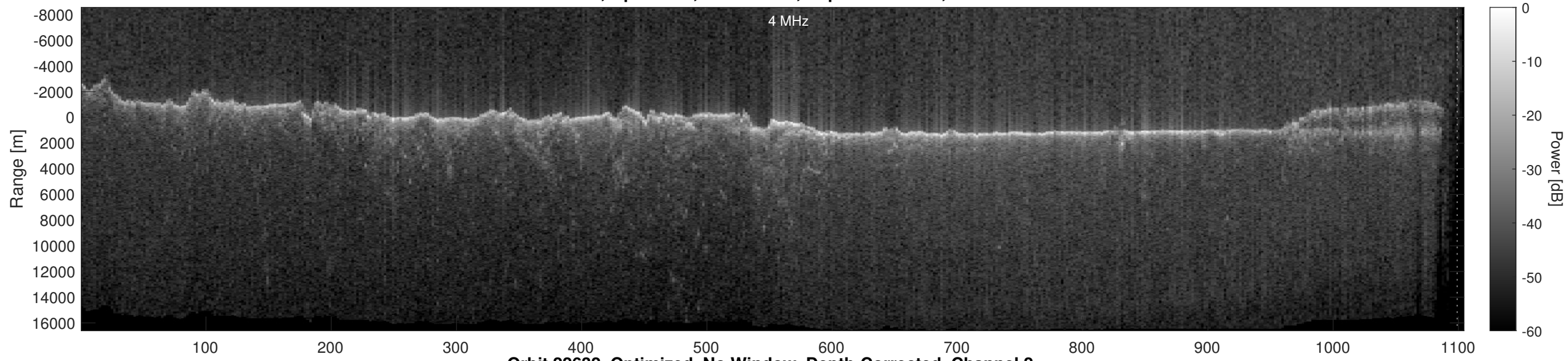
Orbit 22632, Optimized, No Window, Depth-Corrected, Channel 2
