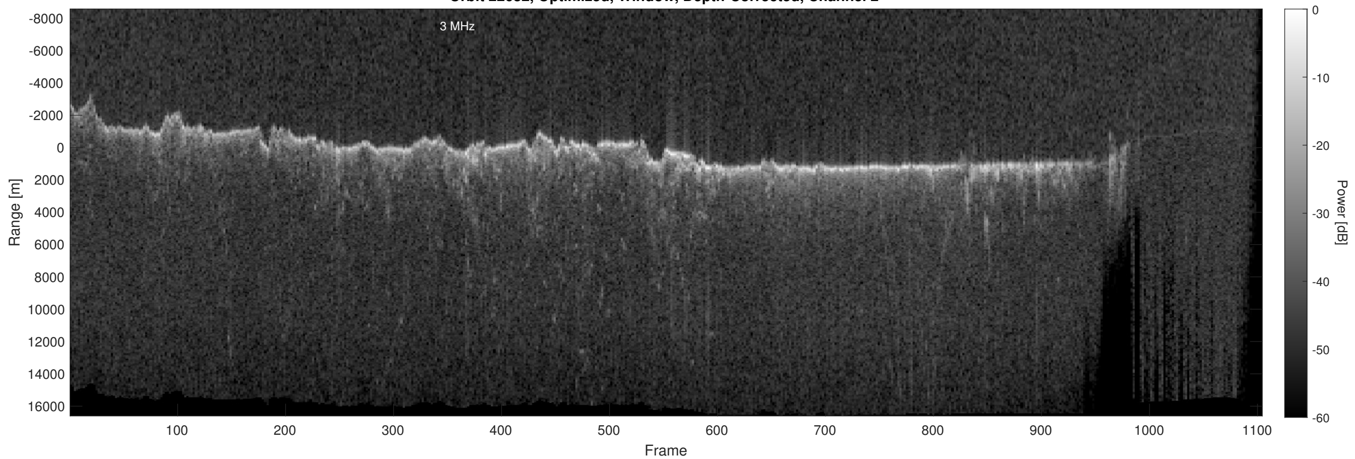
Orbit 22632, Optimized, Window, Depth-Corrected, Channel 2
