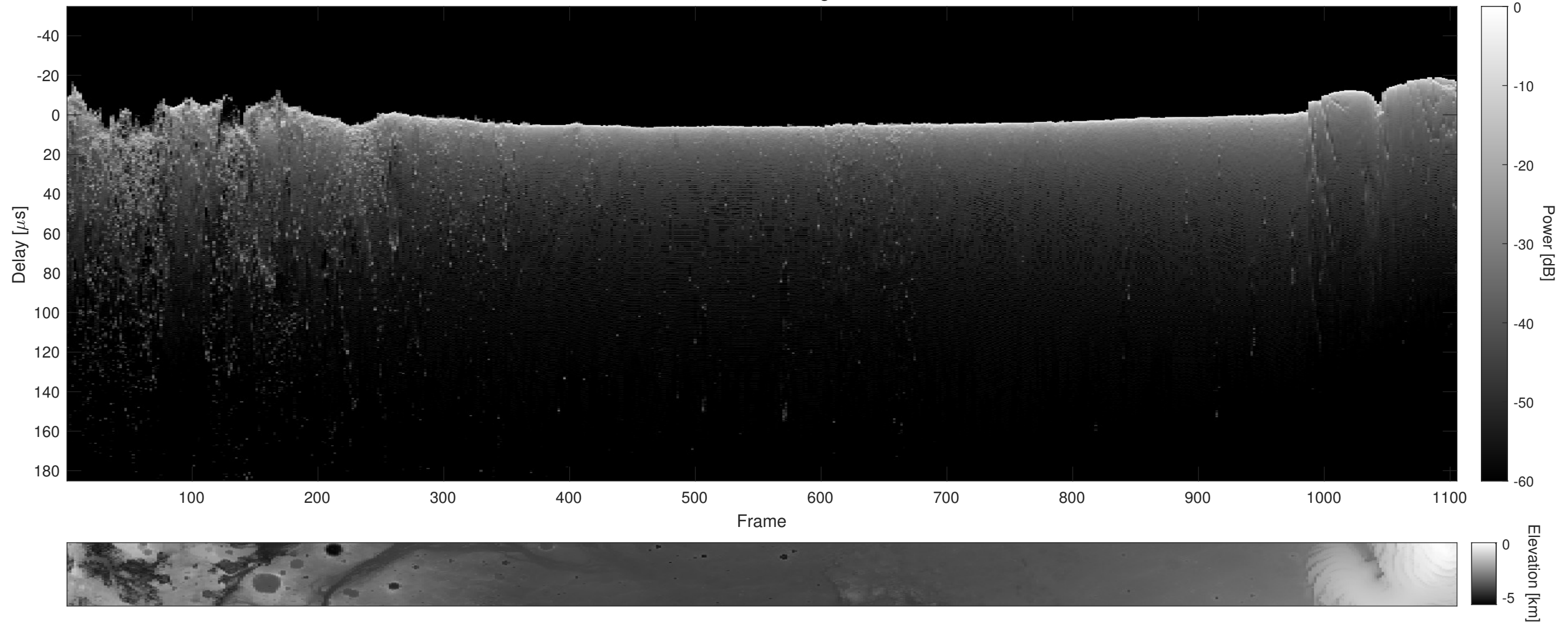
Orbit 22643, Cluttergram
