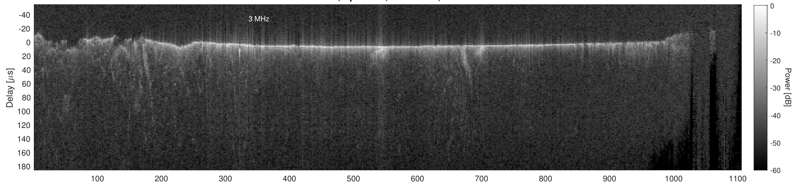
Orbit 22643, Cluttergram
