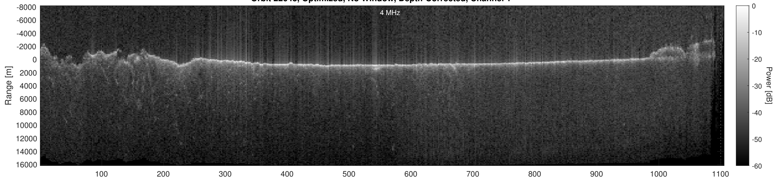
Orbit 22643, Optimized, No Window, Depth-Corrected, Channel 2
