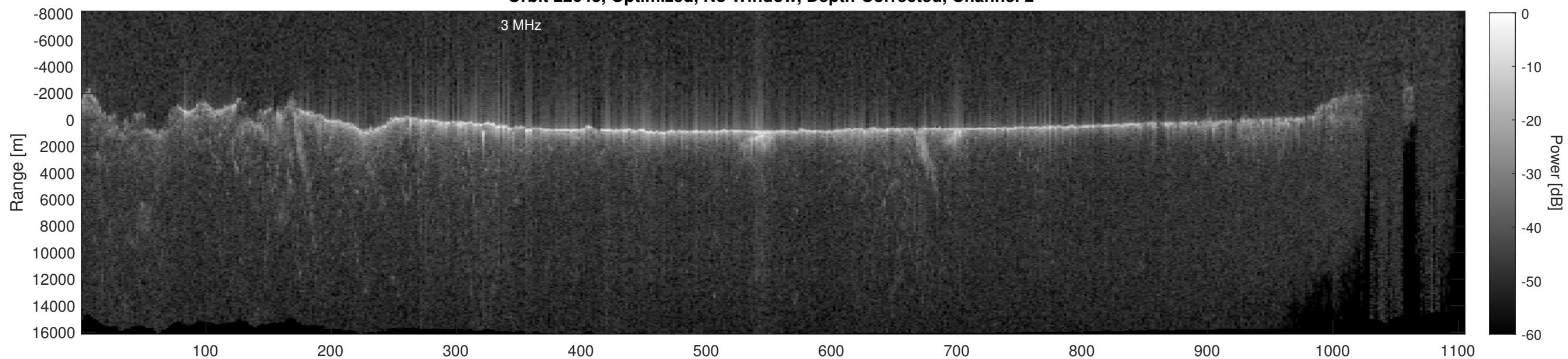
Orbit 22643, Depth-Corrected Cluttergram
