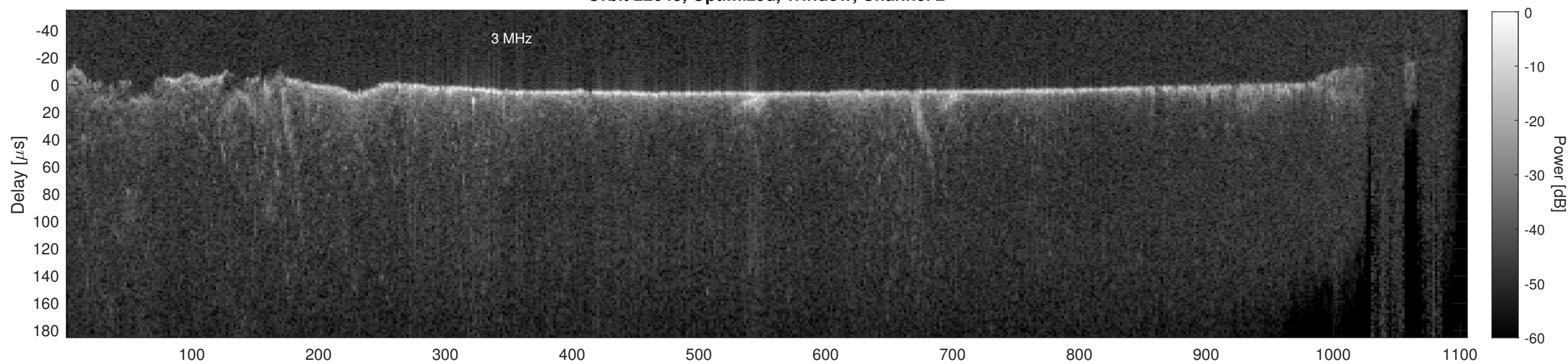
Orbit 22643, Cluttergram
