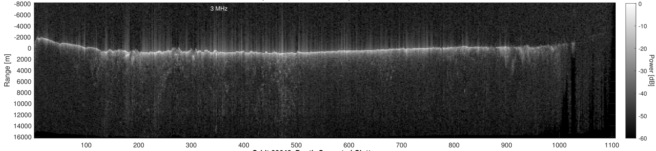
Orbit 22648, Depth-Corrected Cluttergram
