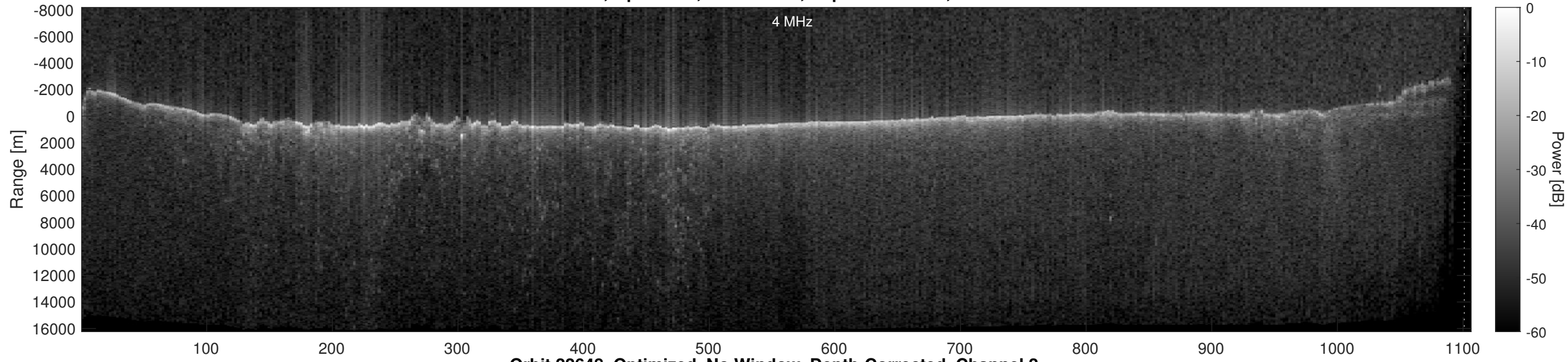
Orbit 22648, Optimized, No Window, Depth-Corrected, Channel 2
