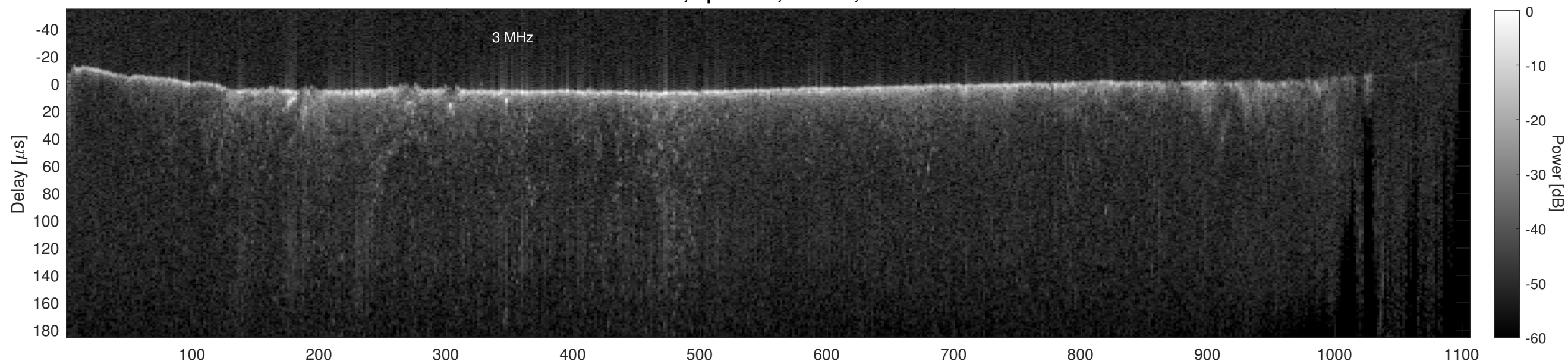
Orbit 22648, Cluttergram
