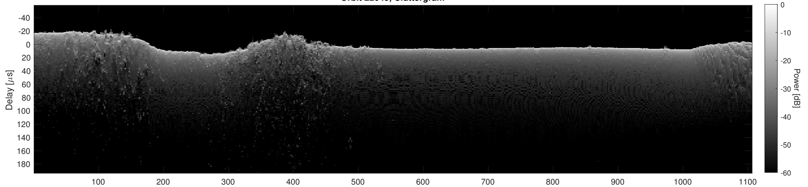
Orbit 22649, Cluttergram
