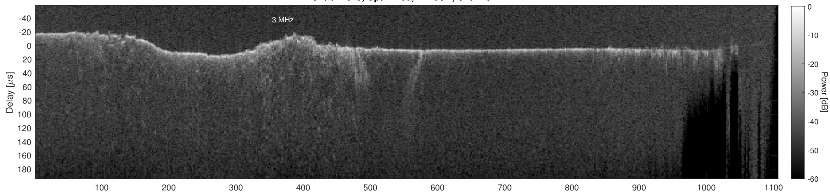
Orbit 22649, Cluttergram
