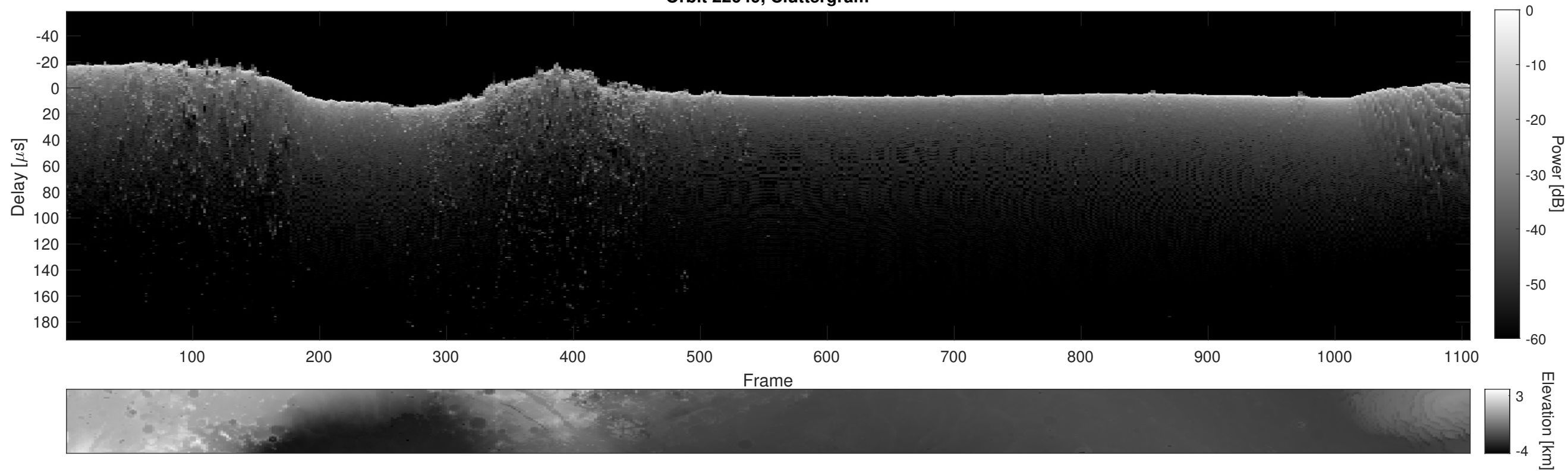
Orbit 22649, Cluttergram
