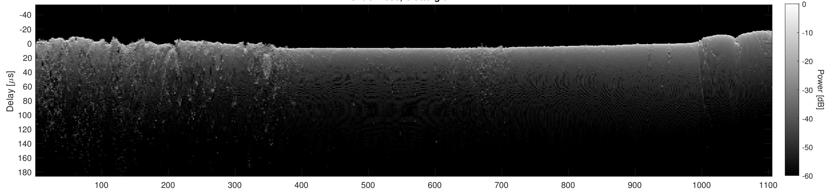
Orbit 22650, Cluttergram
