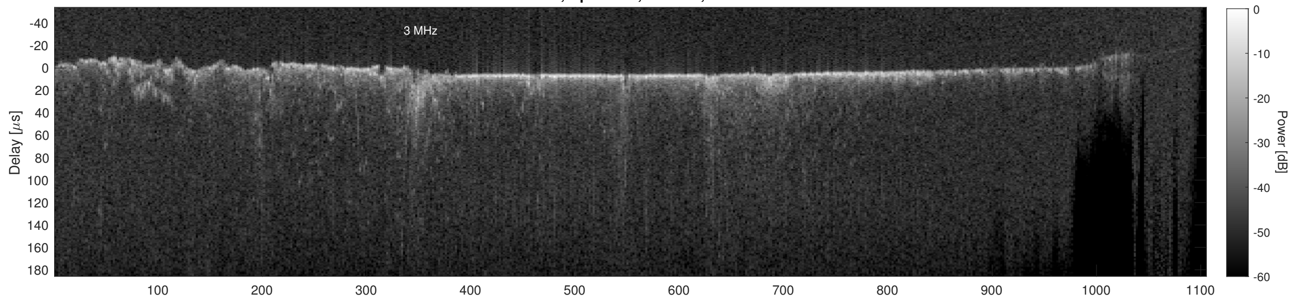
Orbit 22650, Cluttergram
