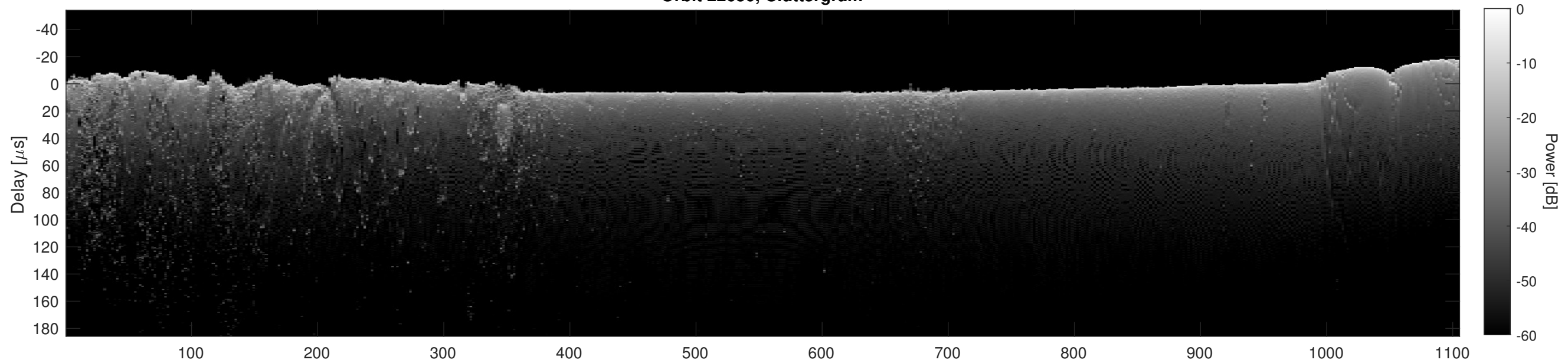
Orbit 22650, Cluttergram
