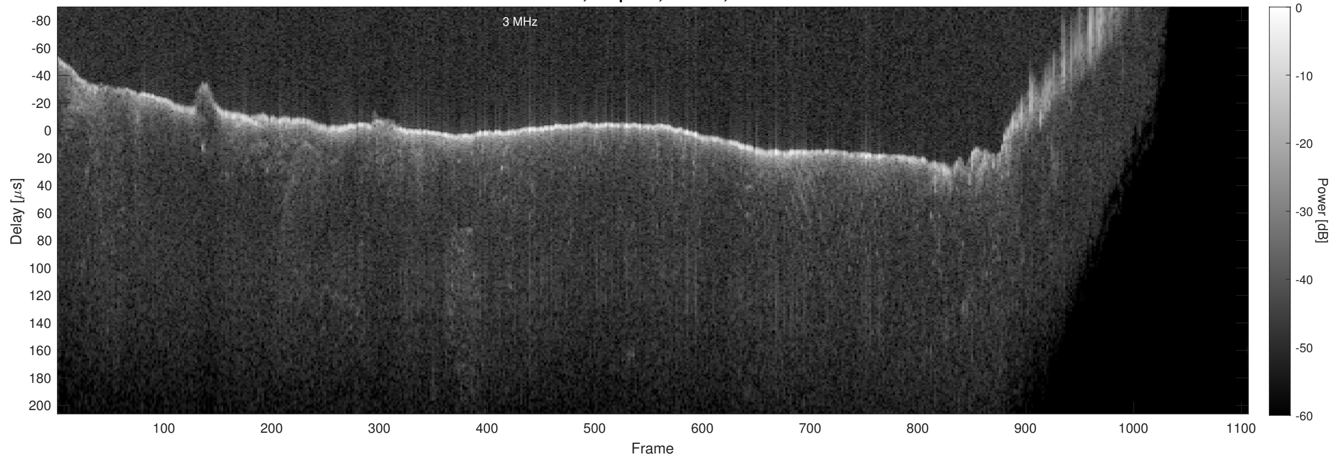
Orbit 22651, Chapman, Window, Channel 2
