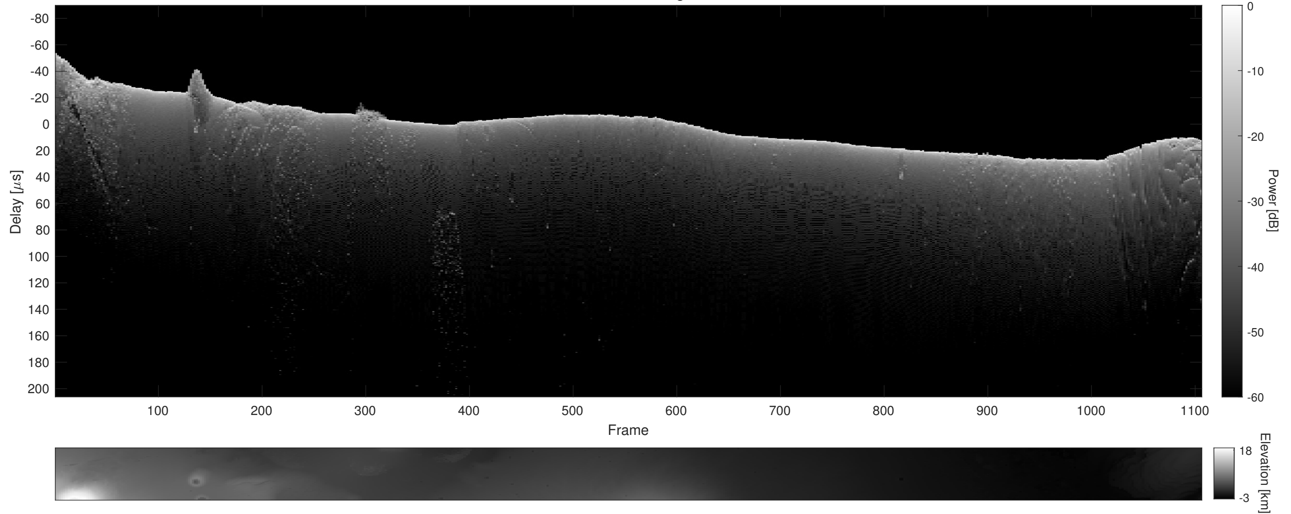
Orbit 22651, Cluttergram
